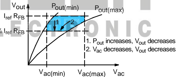
Figure 34. Constant Output Voltage Region
